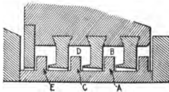
FIG. 97.—Labyrinth bushing.
